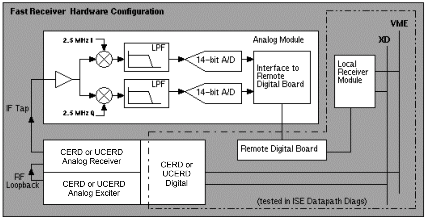
FAST RECEIVER HARDWARE CONFIGURATION ILLUSTRATION 1-1
